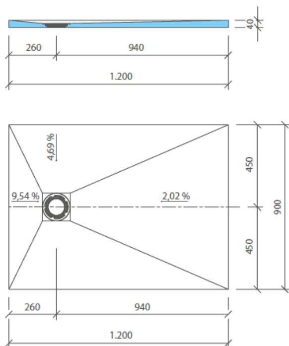
Figure 4 : plan Fundo Primo en 1200x900
